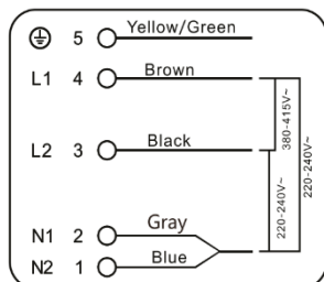
Installation (380V) rare
