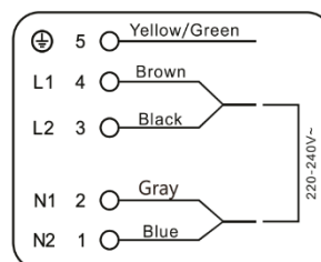
Installation (220V) common
